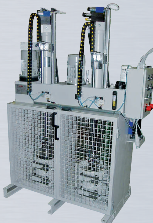
Double pail presses for pigments
