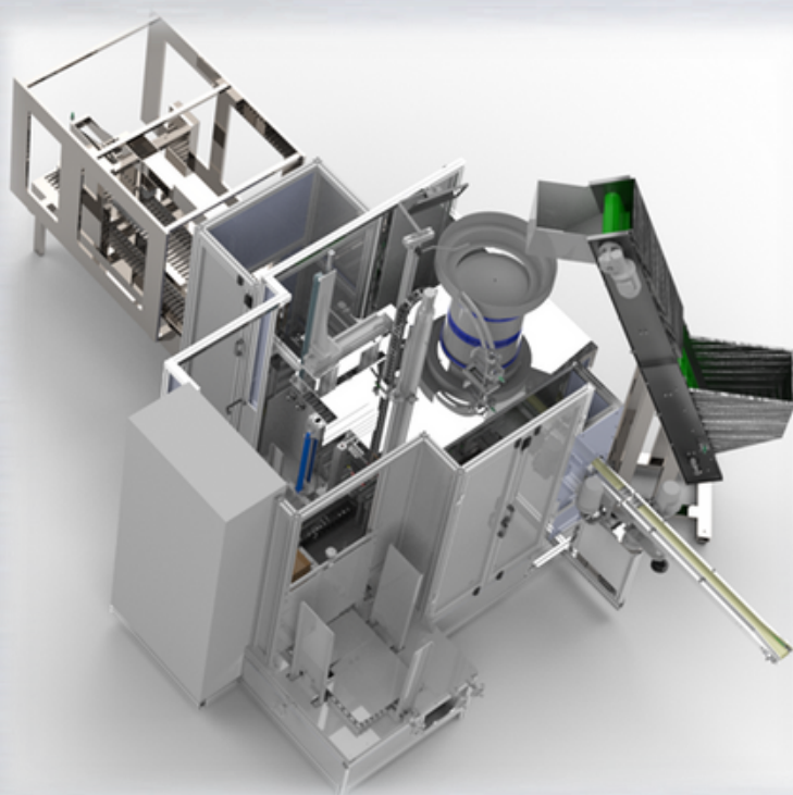
Casepacker type IAC/S for sausages
