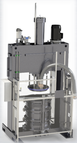
Drum Press type FS180 (80T)
